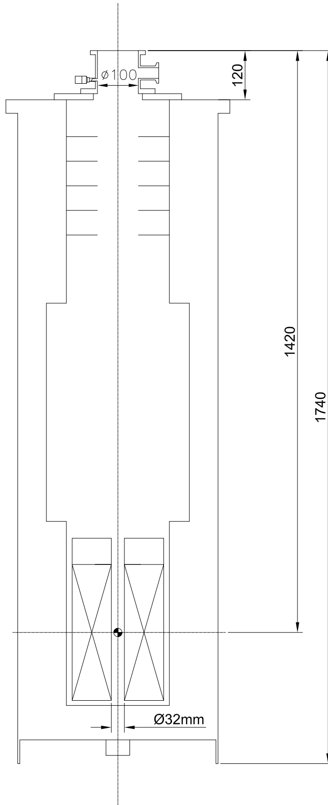
S/C 1 18.5T SUPER CONDUCTING MAGNET (oxford instruments) liquid helium temperature bore= \varnothing 32
