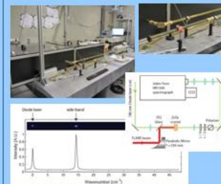
FLARE Diagnostic Station
