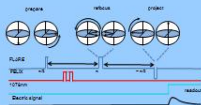
Electrically detected EPR spectroscopy Aeppli, Murdin (London, Surrey)
