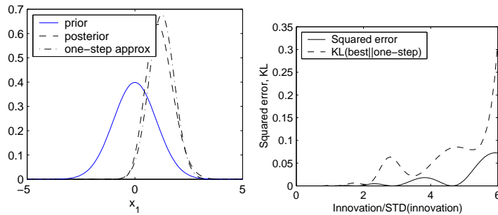
Figure 2: The left plot shows a typical measurement update error; prior x_1 \sim \mathcal{N}(0, 1) (solid), exact posterior p(x_1|y_1 = 3) computed using a very fine grid (dashed), Gaussian approximation from the one-step unscented filter using 5 points (dash-dotted). The mean squared error in the posterior means of such updates and the KL-divergence between best and approximated Gaussian is shown in the right plot as a function of the observation y_t . The x-axis is normalized by the standard deviation of the predictive distribution. The value y = 3 from the left plot corresponds to little over 2 sd.
